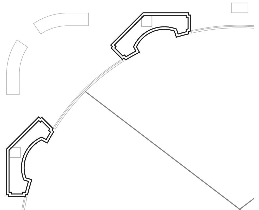
Omaha Court of Appeals 21 Jury Seats - 6'-0" Spacing
